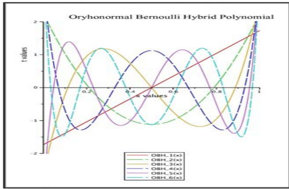
Figure 1: The graph of the first six of Orthonormal Bernoulli Hybrid polynomials.
