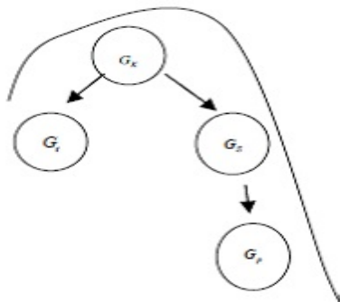
Figure 2: The unique path from G_t to root.
