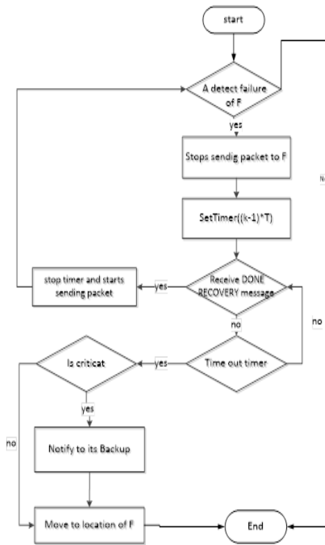
Figure 8: DLA-MRF flowchart
