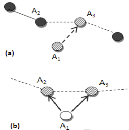
Figure 7: Example of the simultaneous failure of two adjacent nodes (a) the failure of two adjacent critical nodes with the same backup, (b) failure of a critical node and its backup.
