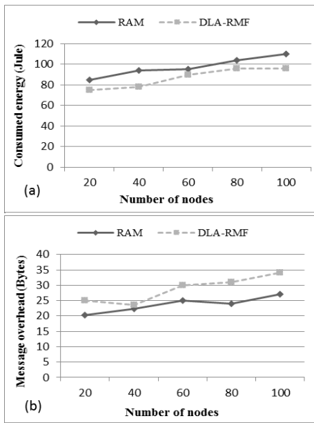
Figure 15: Consumed energy and (b) message overhead during the recovery of DLA-RMF, while varying the network size.
