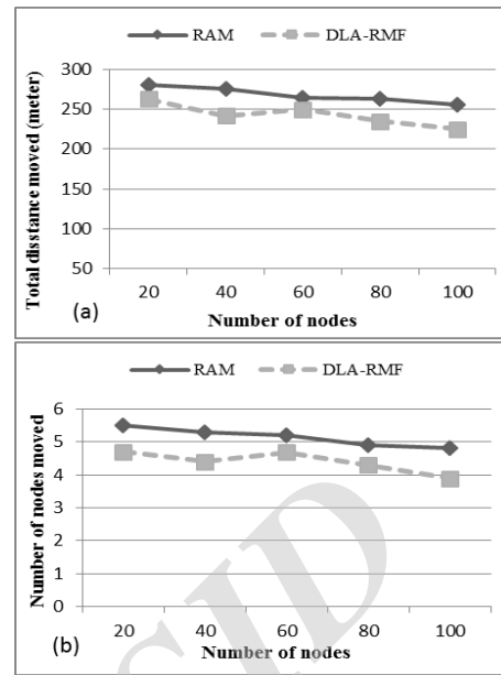
Figure 16: (a) Total distance and (b) number of nodes moved during the recovery of DLA-RMF, while varying the network size.
