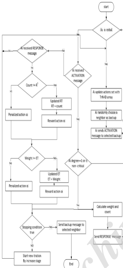
Figure 6: DLA-BuS flowchart
