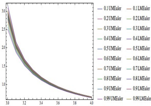
Figure 6: Fuzzy Modified Euler’s Method for example (??)
