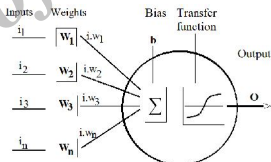
Figure 3. Mathematical representation of a neural cell in the network
