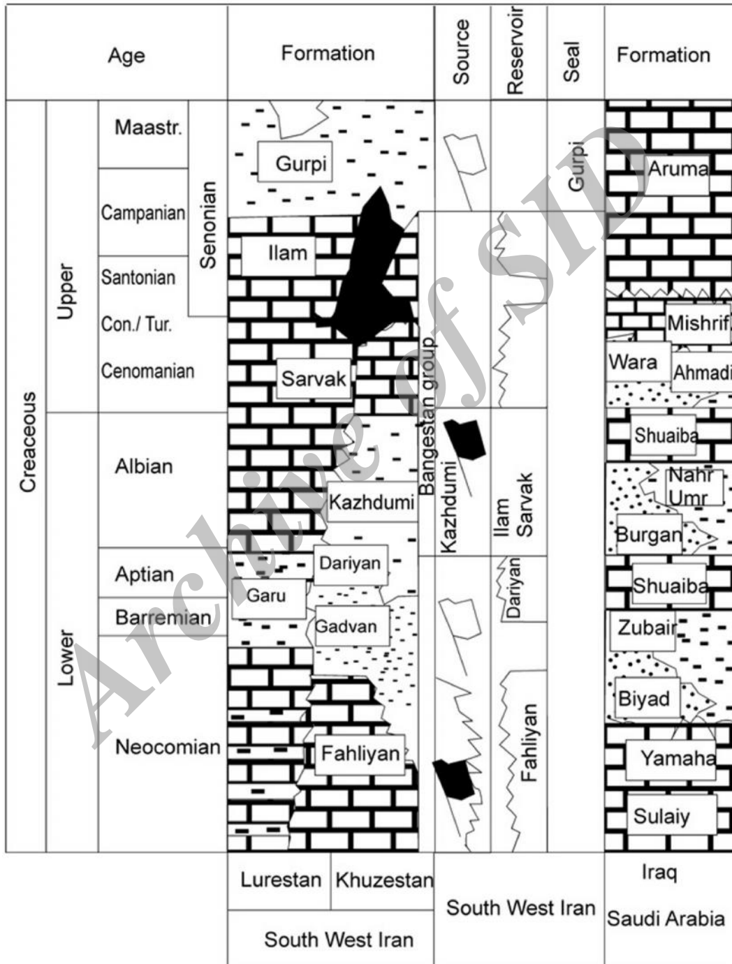
Figure 2. Stratigraphic chart of the Cretaceous system of southwest Iran and adjacent areas (Bordenave, 2002)
