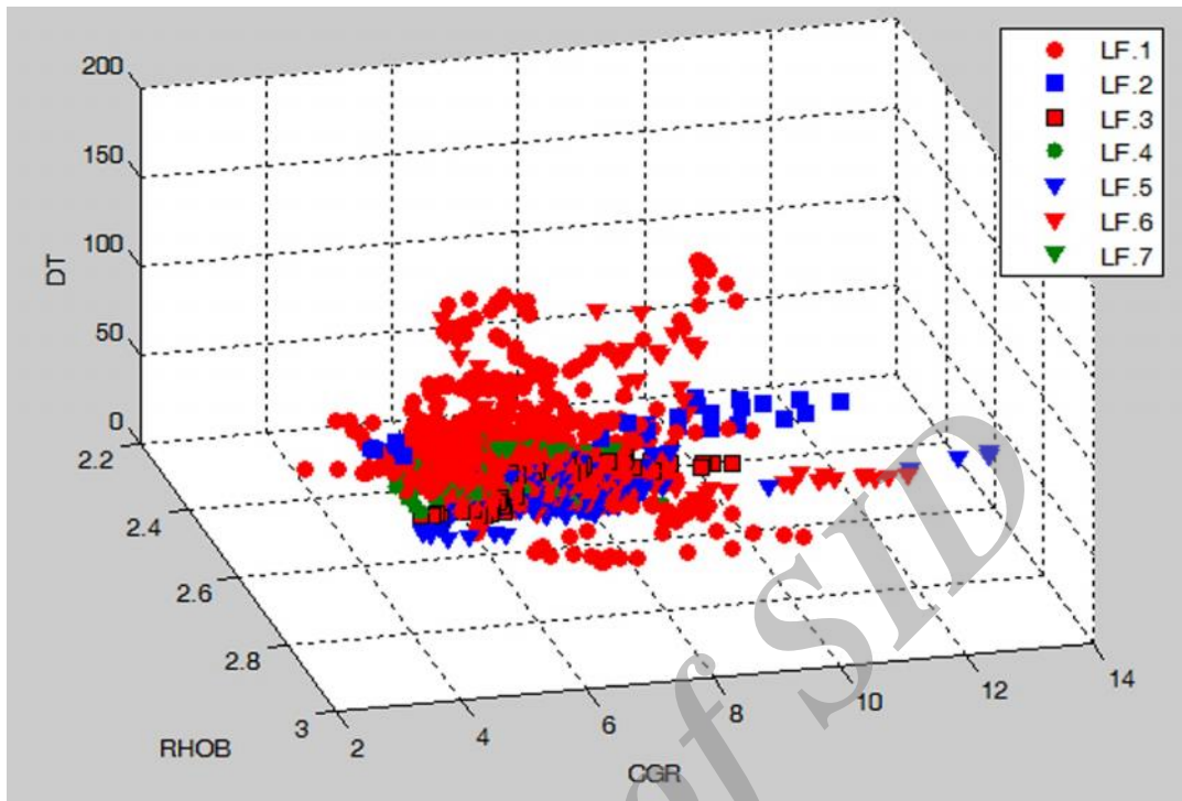
Figure 10. Cross plot of DT vs. RHOB and CGR
