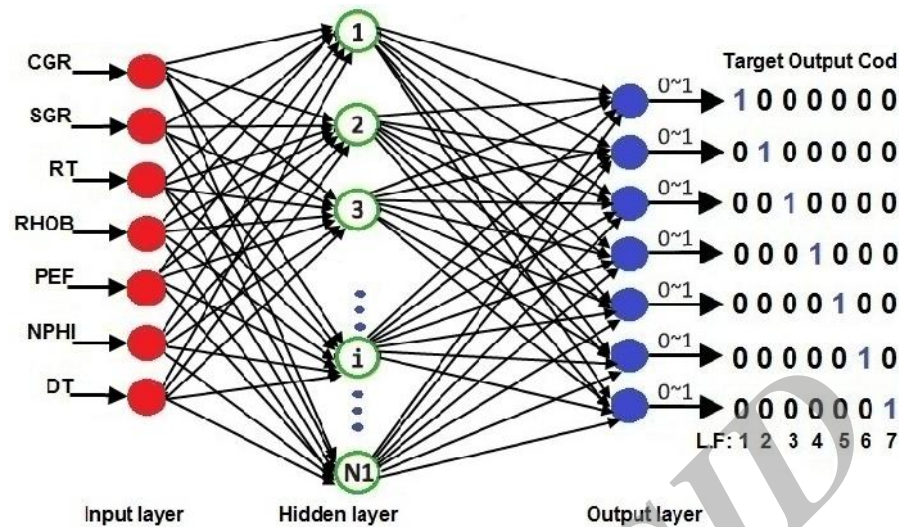
Figure 4. Architecture of the artificial neural network built for this study
