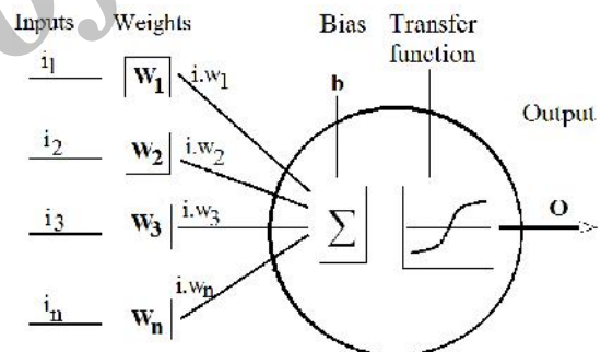
Figure 3. Mathematical representation of a neural cell in the network
