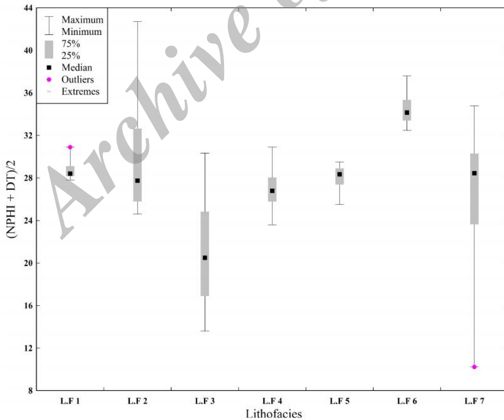
Figure 9. box plot of porosity vs. lithofacies
