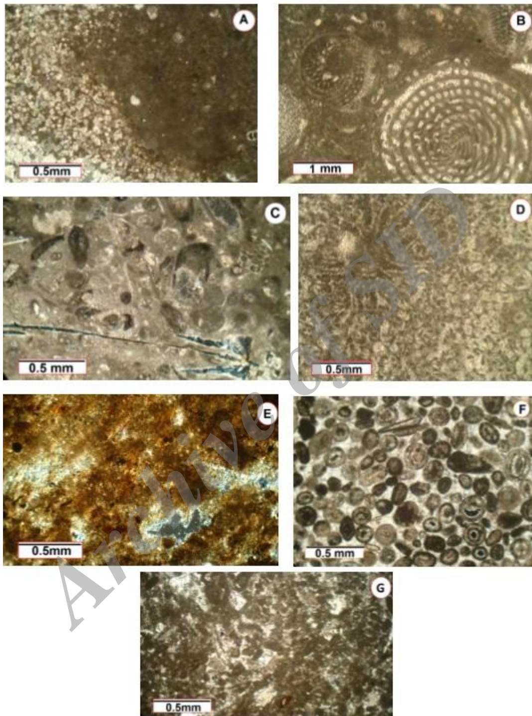
Figure 5. Photomicrograph of seven lithofacies types recognized from Sarvak Fm. in well # 305, Marun oil field (A) dolomudstone; (B) floatstone; (C) wackestone; (D) boundstone, (E) mudstone, (F) ooid grainstone and (G) packstone
