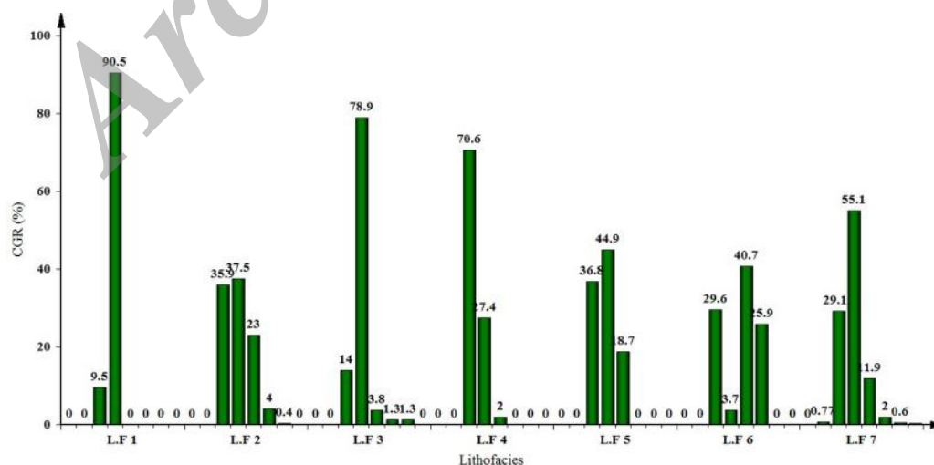
Figure 7. Histogram of CGR vs. lithofacies
