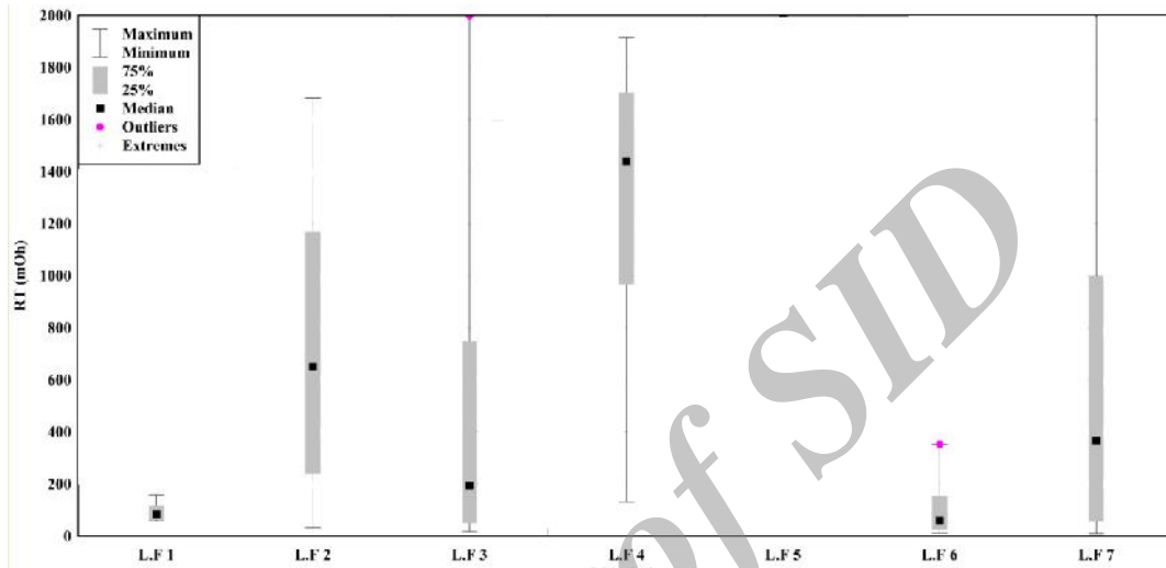
Figure 8. box plot of RT and porosity vs. lithofacies
