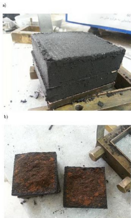
Figure 15. Direct shear test; a) a treated sample by NZVI at the end of the test, b) transformation of \text{Fe}^0 to \text{Fe}^{2+} (orange spots) due to the mentioned reactions
