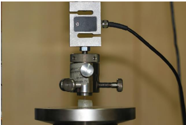
Fig. 3: Push-out test
