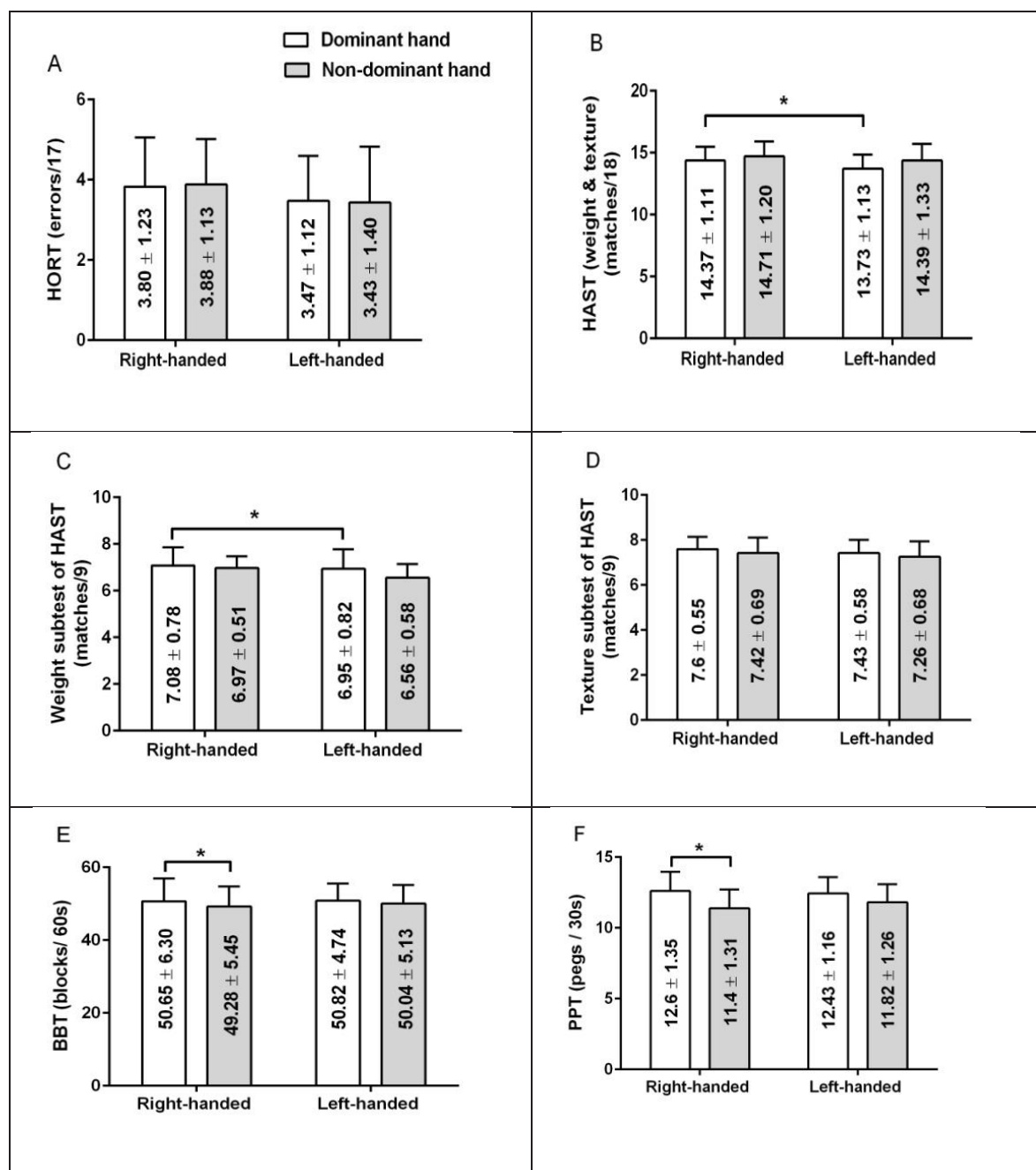
Figure 1. The results of multiple comparisons for interaction between laterality and handedness in sensory-motor functions of the elderly participants (* P \leq 0.05 )
