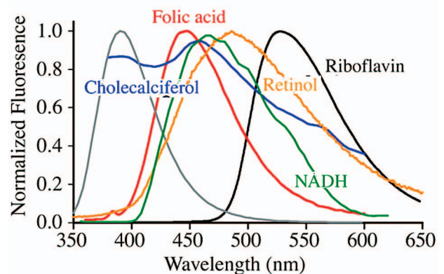
Figure 5. Emission spectra of some biological components. All compounds were measured in buffered (pH 7.2) saline solution, except retinol and cholecalciferol (vit D), which were measured in EtOH. Riboflavin, cholecalciferol, and NADH were measured at 100 μM; retinol, folic acid, phyloquinone, pyridoxine, and nicotinamide were measured at 500 μM. (b) Emission spectra of the compounds shown in a (measured in the same solvents) (41).
