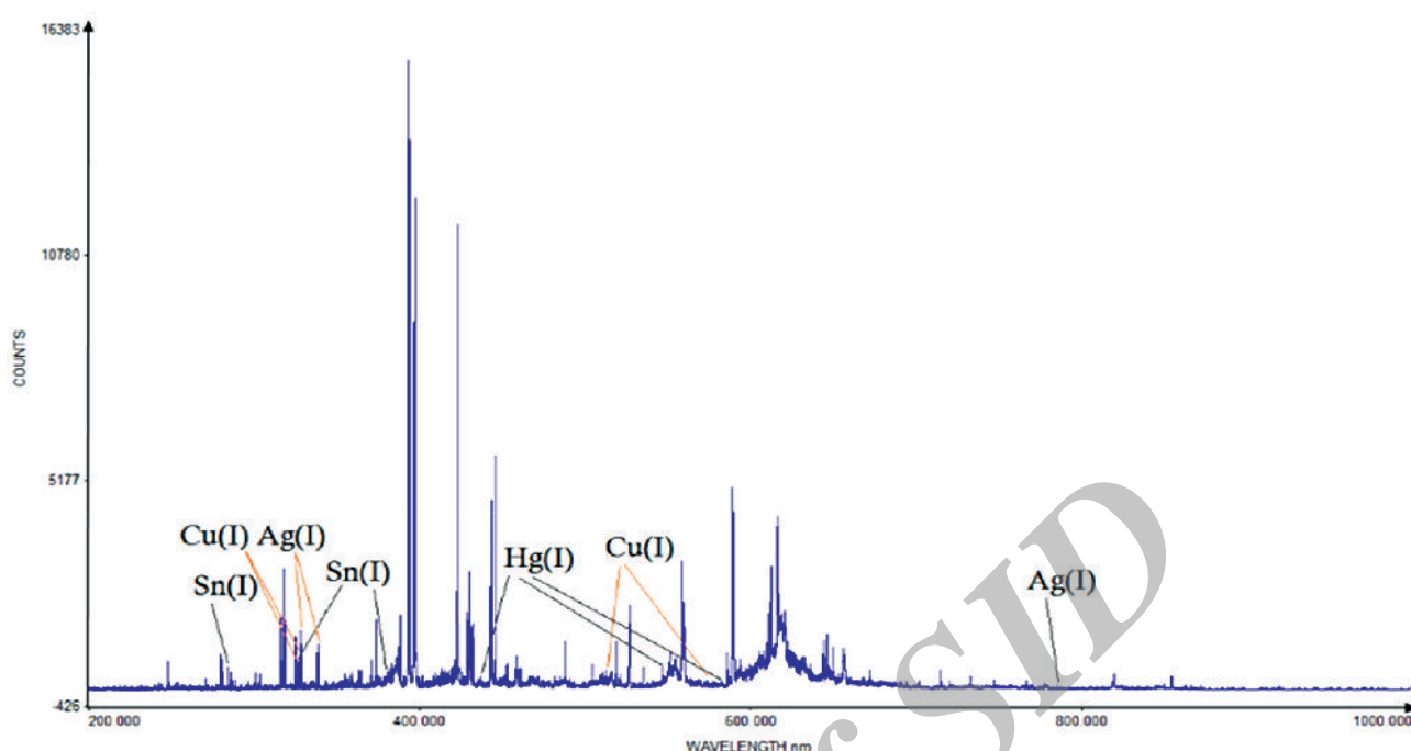
Figure 7. LIBS spectrum of amalgam filled tooth.
