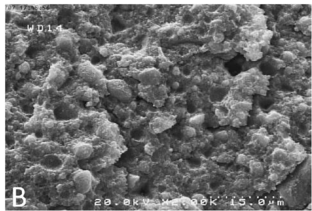
Figure 5 (A, B). Surface treated by Er:YAG laser with power of 5 W, 250 mJ (Original magnification x500, x2000)
