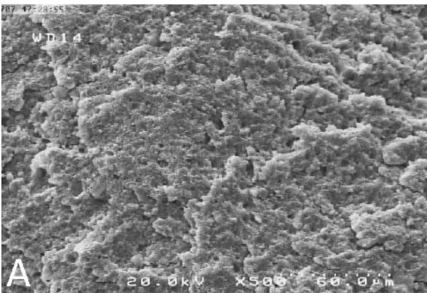
Figure 3 (A, B). Surface treated by Er:YAG laser with power of 3 W, 150 mJ (Original magnification x500, x2000)
