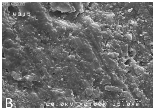
Figure 6 (A, B). Surface treated by Er:YAG laser with power of 6 W, 300 mJ (Original magnification x500, x2000)
