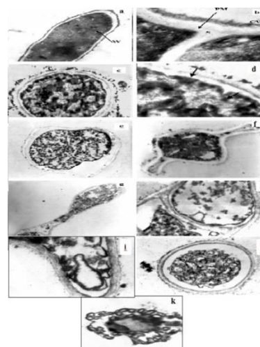
Figure 1. Transmission electron micrographs of Aspergillus species (CW: Cell wall; PM: Plasma membrane; S: Septum; W: Woronin body).
