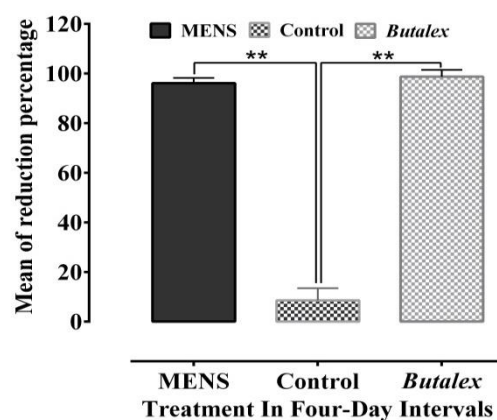
Figure 3. Mean of reduction percentage of parasitemia rates following treatment with N. sativa methanolic extract (MENS) and Butalex ®. Significant differences have been shown at ** p < 0.001 . Values are reported as Mean±SEM.
