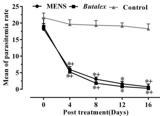
Figure 1. Changes in parasitemia rates following administration of N. sativa methanolic extract (MENS) and Butalex ® compared to control. Data are presented as mean±SEM (n=30). *Significant differences ( p < 0.05 ) between the control group versus MENS and Butalex ® groups. +Significant differences ( p < 0.05 ) between various days of each group. No significant difference was observed between MENS and Butalex groups.
