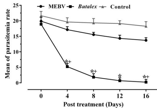
Figure 2. Changes in parasitemia rates following administration of B. vulgaris methanolic extract (MEBV) and Butalex ® compared to control. Data are presented as mean±SEM (n=30). *Significant differences ( p < 0.05 ) between the Butalex ® group versus control and MEBV groups. +Significant differences ( p < 0.05 ) between various days of each group. No significant difference was observed between groups MEBV and Control.
