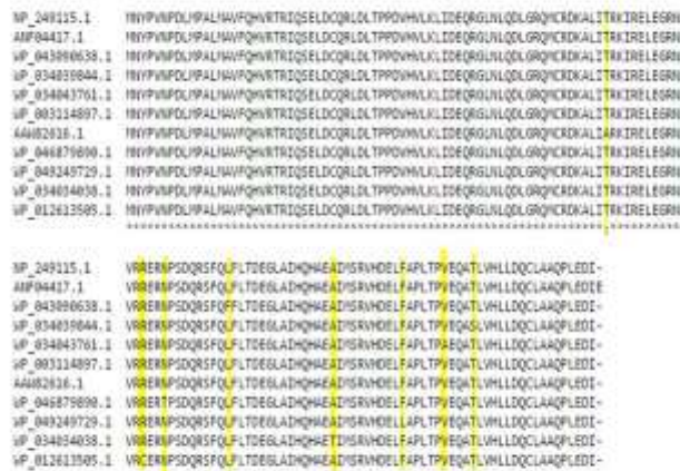
Figure2- Secondary structure prediction by ESPrict depicted alpha helix regions in MexR
