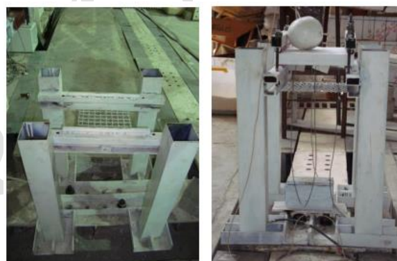
Fig. 2. Details of impact test support
