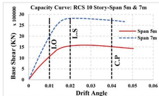
Fig. 4 Capacity curve of RCS 10 story
