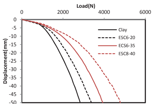
Fig 2. Load settlement variations of encased stone columns
