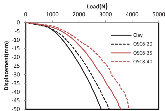
Fig 1. Load settlement variations of ordinary stone columns
