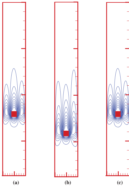
Fig. 2. stream lines near the square cylinder in channel filled with shear-thinning ( n=0.9 ), Newtonian ( n=1.0 ), and shear-thickening fluids ( n=1.1 ), Ar_{pi}=10^3 .
