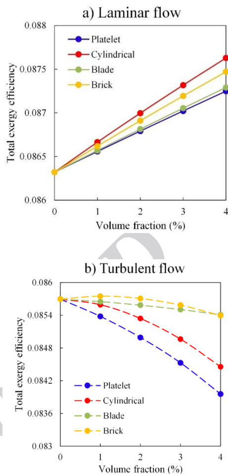
Fig.2. Variation of total exergy efficiency with volume fraction for different nanoparticle shapes in laminar and turbulent regimes.
