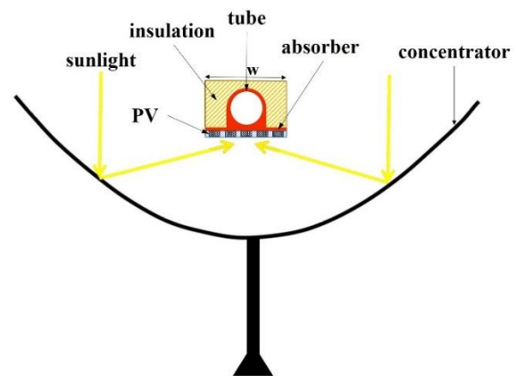
Fig. 1. Concentrating photovoltaic/thermal system.
