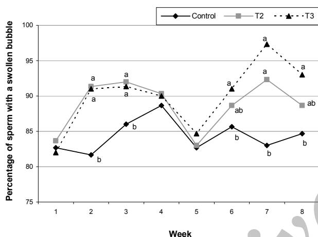
Fig. 1: Effect of diet \times time (week) interaction on the percentage of sperm with a swollen bubble around the curled flagellum in a hypotonic solution (HOS) in roosters fed Satureja khuzistanica powder (pooled SE = 1.8745). Satureja khuzistanica powder was included at 0 (T1 or control), 20 g (T2), or 40 g (T3) per kg diet for 8 weeks. a, b: The means with different superscripts in each row differ significantly ( P < 0.05 ). No differences were found at week 1, 4 and 5
