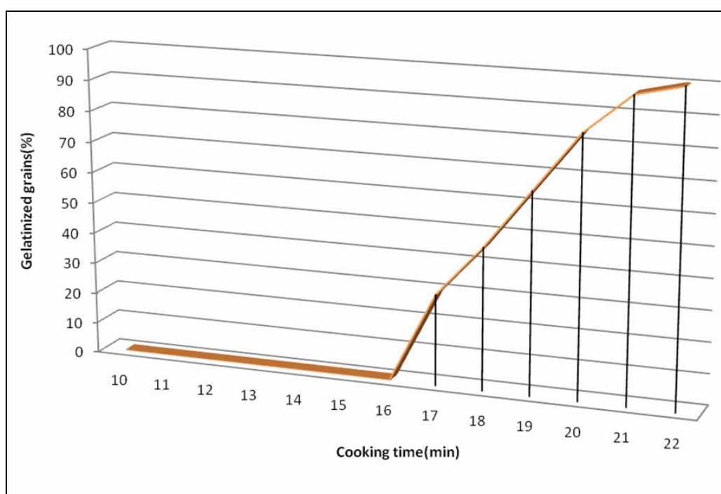
Fig. 2. Gelatinization profile of HD5 rice samples
