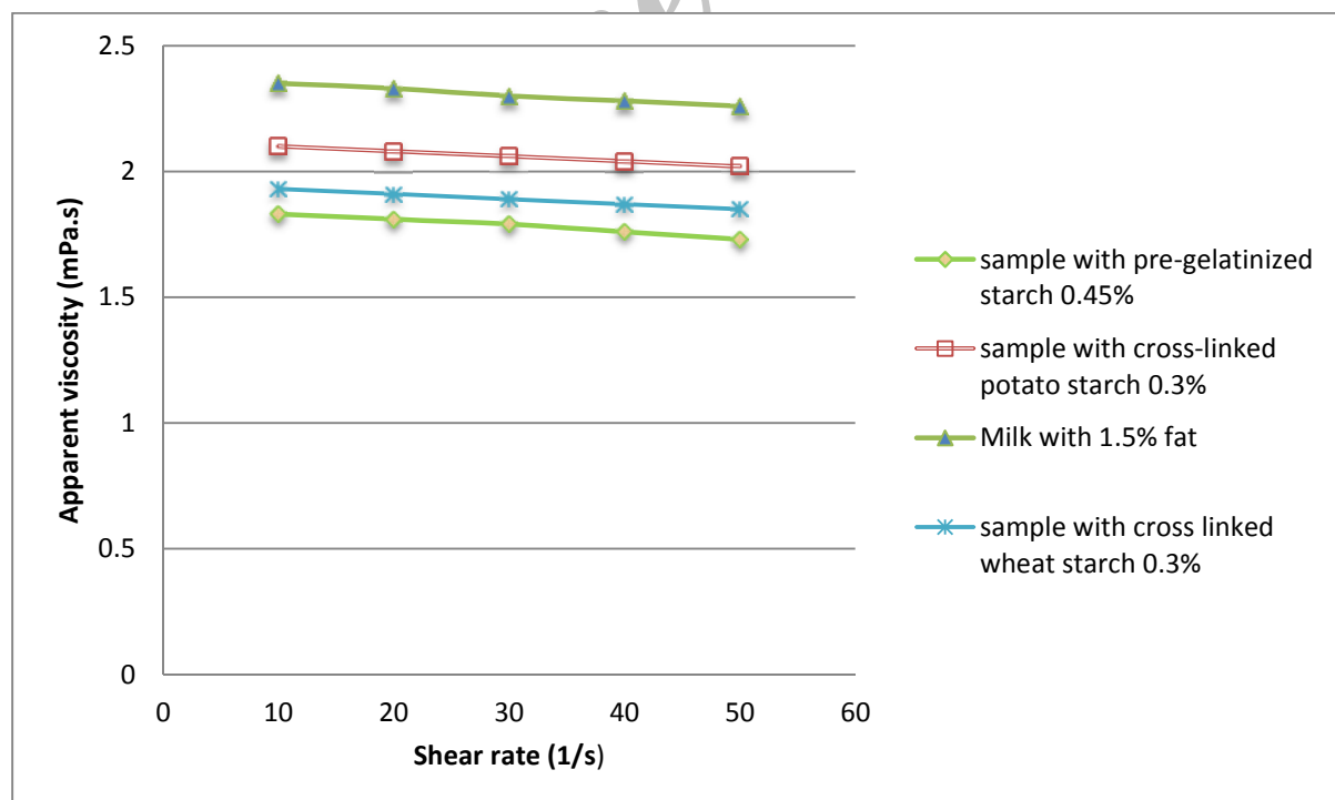
Fig. 1. Viscosity versus shear rate plot of milk samples at 25°C
