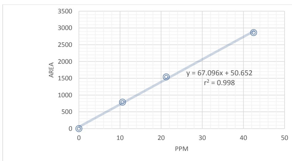
Fig. 1. The calibration curve indicating the acrylamide concentration against the area of the peak by HPLC
