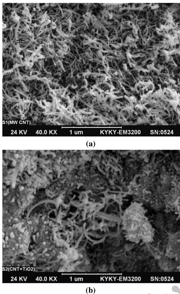
Figure 2. SEM image of (a) f-MWNT, (b) MWNT/TiO 2 hybrid.
