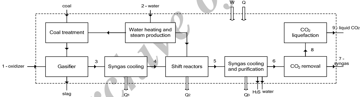
Fig. 7: Coal decarbonization process
