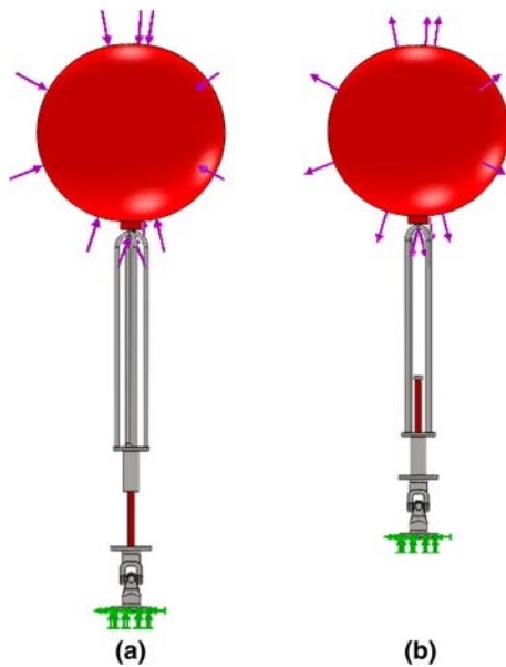
Fig. 6 Boundary and applied load conditions for two extreme stroke positions of hydraulic cylinder piston rod: a position A and b position B
