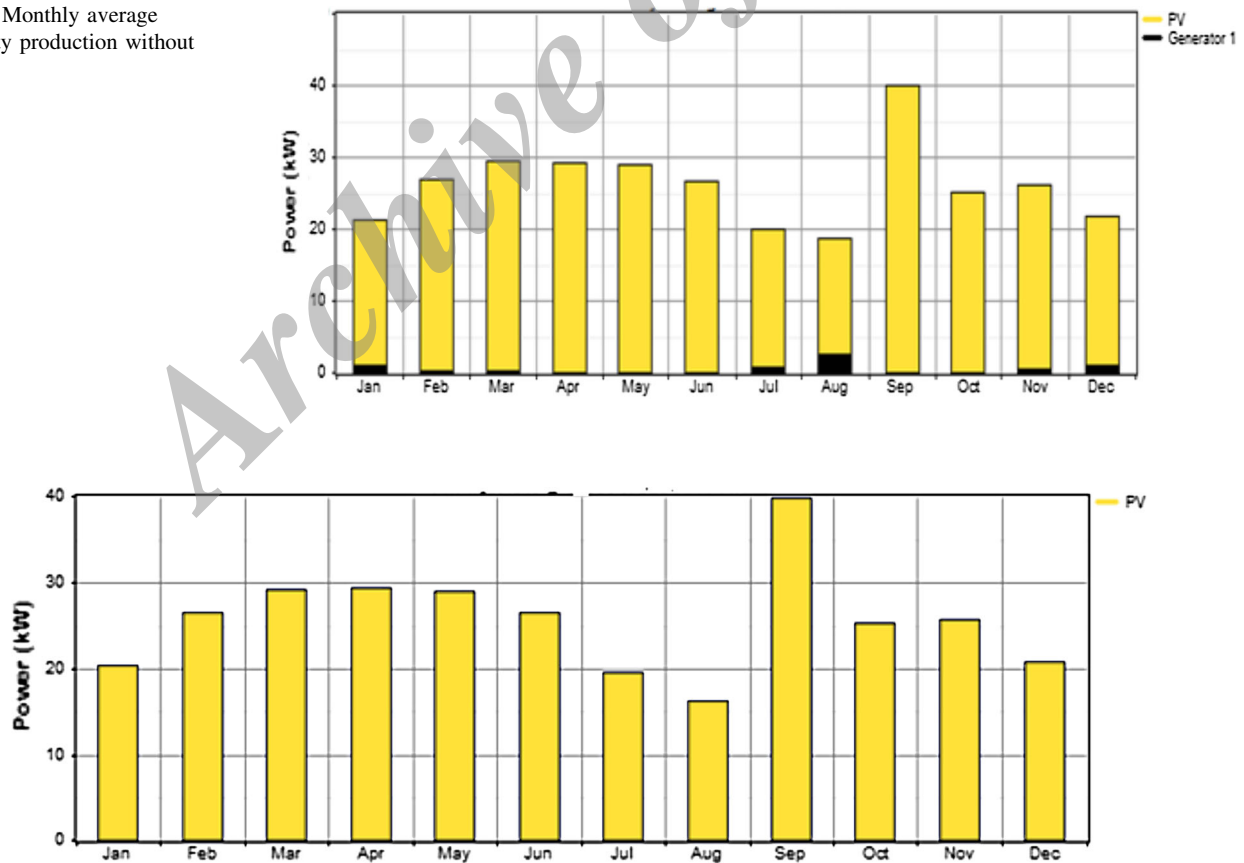
Fig. 11 Monthly average electricity productions with DSM
