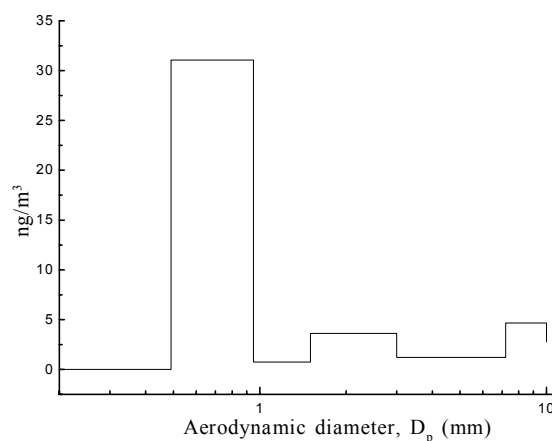
Fig. 5: Size distribution of PAH s at Haft-Houz Square
