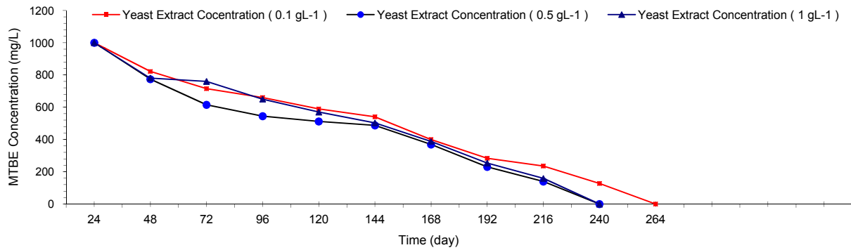
Fig. 1: MTBE biodegradation by microbial consortium in the presence of different concentrations of yeast extract
