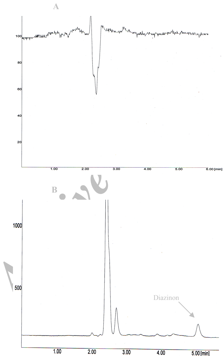
Fig. 1 Chromatograms obtained before and after MISPE. A: before MISPE of LC-grade water spiked with 50 ng/mL of diazinon. B: after MISPE of 10 mL of LC-grade water spiked with 50 ng/mL of diazinon. C: after MISPE of drinking water (500 mL) spiked with 1 ng/mL of diazinon.
