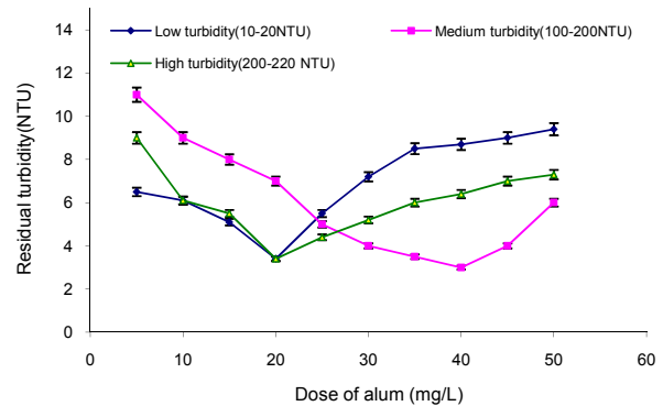
Fig2 : Determination of optimum dose of alum in different turbidities
