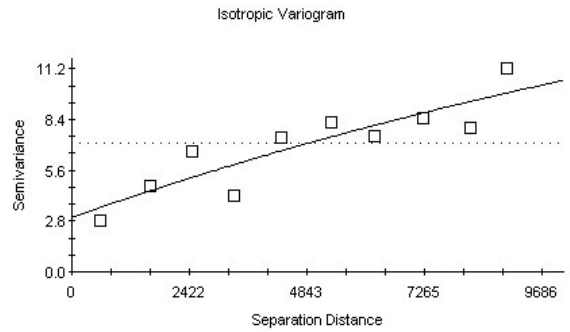
Fig. 3: Exponential semi-variogram model \gamma(h;\theta) fitted to classical semi-variogram estimate \hat{\gamma}(h) in different distances with GLS method for EC dataset in May 2009
