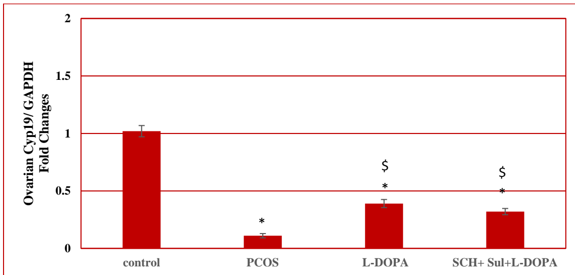
Chart 2. Effects of L-DOPA or simultaneous injections of R (+) SCH23390, sulpiride and L-DOPA on aromatase ( Cyp19 ) gene expression in the ovary of PCOS rats. *: compared to control; $: compared to PCOS; #: compared to L-DOPA.
