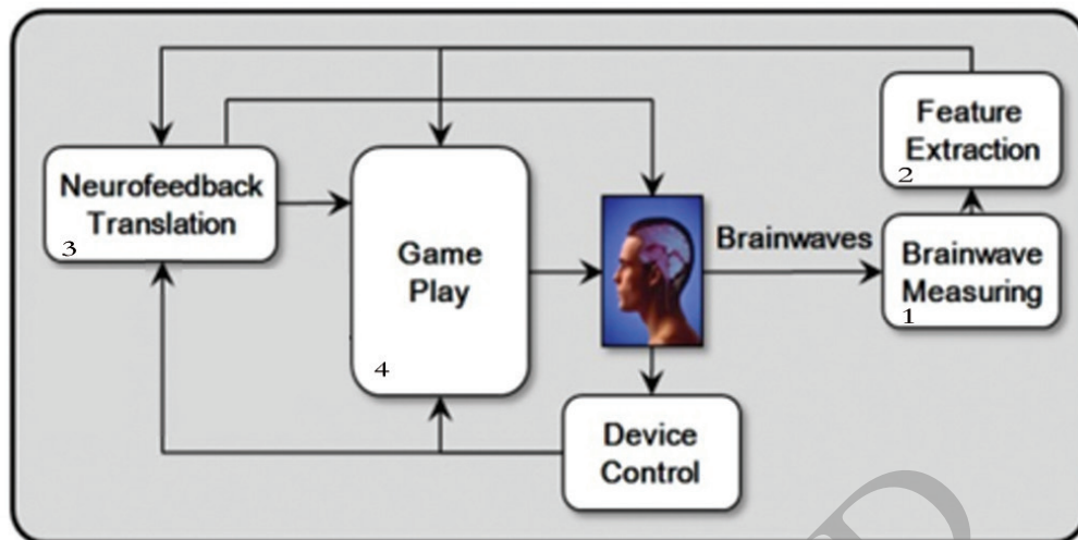
Figure 1. The stages of neurofeedback training: 1. Measuring brainwaves 2. Extraction of patterns and distribution of alpha and theta waves in O1 and O2 3. Transformation of brain waves into feedback (eg. game play) 4. Monitoring of feedbacks by subjects. In all stages, neurofeedback device control the process of game play transforming brain waves to feedbacks.
