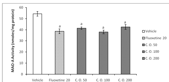
Figure 3. Effect of Celastrus paniculatus seed oil on MAO-A levels.
