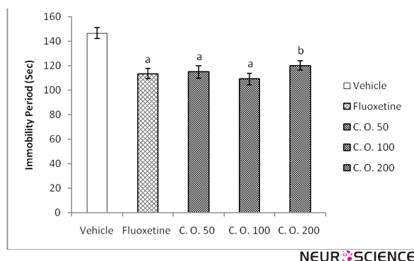
Figure 1. Effect of Celastus paniculatus seed oil on immobility period using FST.
