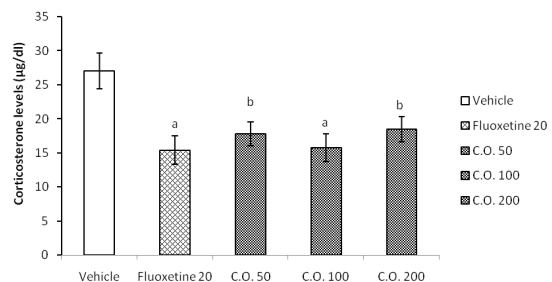
Figure 4. Effect of Celastrus paniculatus seed oil on corticosterone levels.
