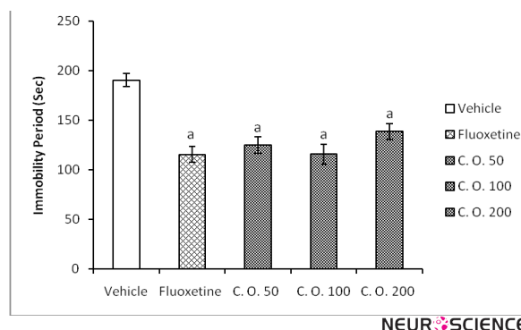
Figure 2. Effect of Celastus paniculatus seed oil on immobility period using TST.
