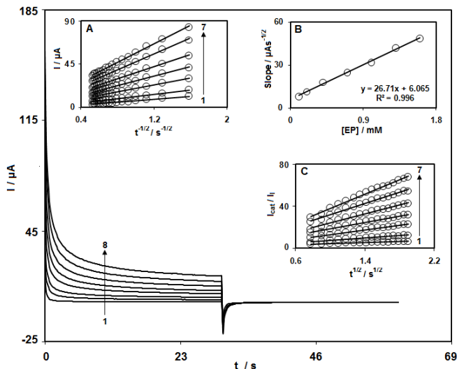
Fig. 5. Chronoamperograms obtained at DDP-CPE in 0.1 M phosphate buffer solution (pH 7.0) for different concentrations of EP. The numbers 1–8 correspond to 0.0, 0.1, 0.2, 0.4, 0.7, 1.0, 1.3 and 1.6 \text{mM} of EP. Insets: (A) Plots of I vs. t^{-1/2} obtained from chronoamperograms 2–8. (B) Plot of the slope of the straight lines against EP concentration. (C) Dependence of I_{\text{cat}}/I_1 on t^{1/2} derived from the data of chronoamperograms 1–8.
