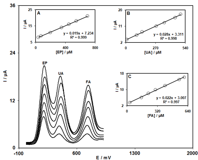
Fig. 6. DPVs of DDP-CNPE in 0.1 M phosphate buffer solution (pH 7.0) containing different concentrations of EP+UA+FA in μM, from inner to outer: 40.0+10.0+30.0, 75.0+100.0+150.0, 200.0+150.0+225.0, 350.0+275.0+300.0, 450.0+350.0+400.0, 550.0+450.0+550.0 and 700.0+500.0+600.0, respectively. Insets (A) (B) and (C) are plots of I_p vs. EP, UA and FA concentrations, respectively.
