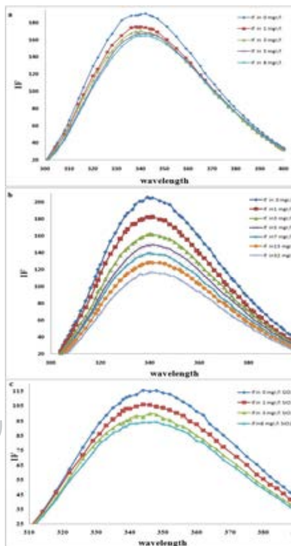
Fig. 3. Fluorescence quenching of lysozyme, \lambda_{\text{exi}} = 280 nm in the presence of various concentration of SiO 2 at (a) pH = 2.5, (b) pH = 7.25, (c) pH = 11.
