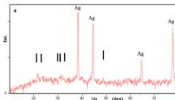
Fig. 5. XRD pattern of the Ag-CNTs electrode after some C&D cyclic Li storage and marked peaks belong to Li_2CO_3 precipitate. This is an indicative for formation of the SEI film [6]
