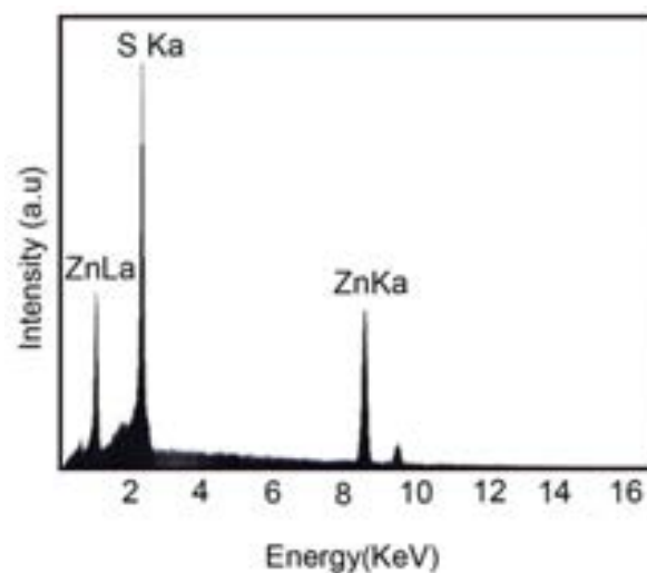
Fig. 6. EDX analysis of ZnS nanoparticles.
