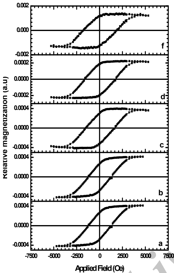
Fig. 7. The hysteresis loops of CoNi nanowire arrays with applied field parallel to the nanowire with the reductive \square oxidative time of 1ms and off-times of (a) 20ms, (b) 50ms, (c) 100ms, (d) 200ms and (f) 400ms.
