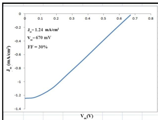
Fig. 9. I–V characterisation of the solar cell of the obtained CuInS 2 with TSC at 8 h.
