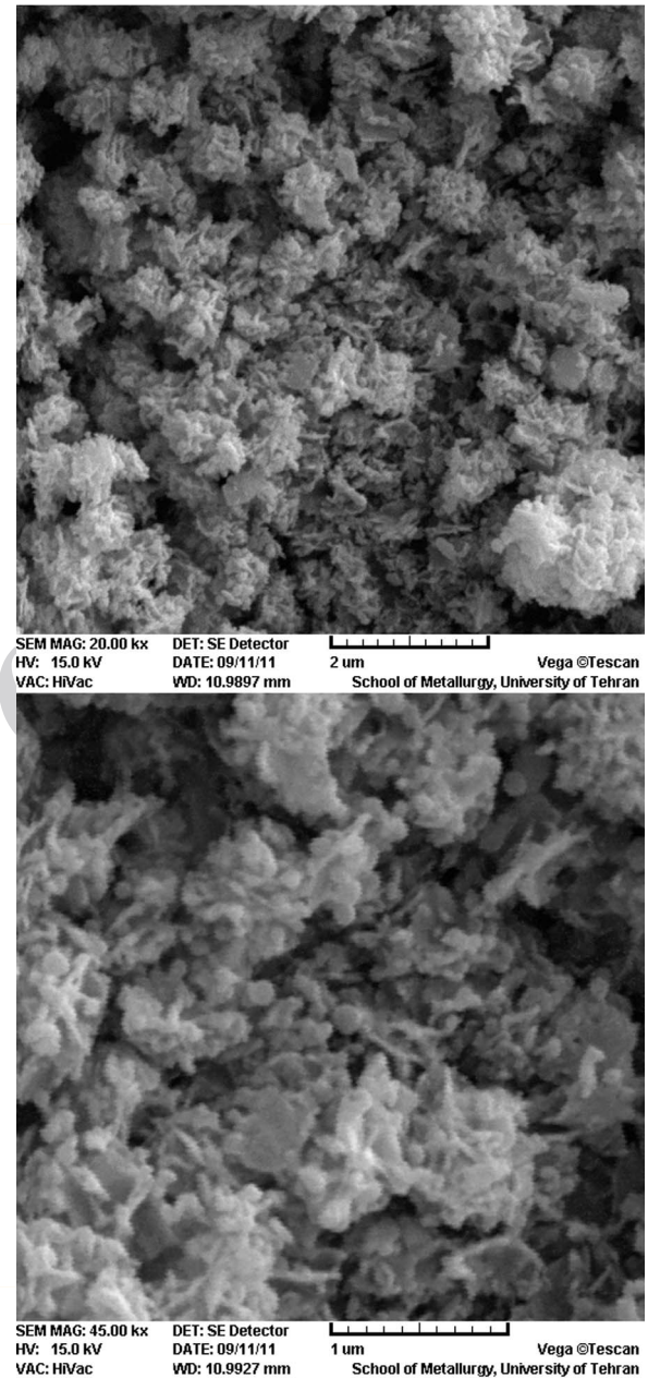
Fig. 5. SEM images of the obtained CuInS 2 with thioglycolic acid at 8 h.
