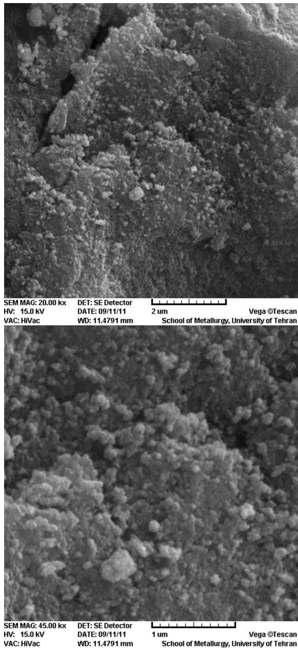
Fig. 4. SEM images of the CuInS 2 with TSC at 10 h.
