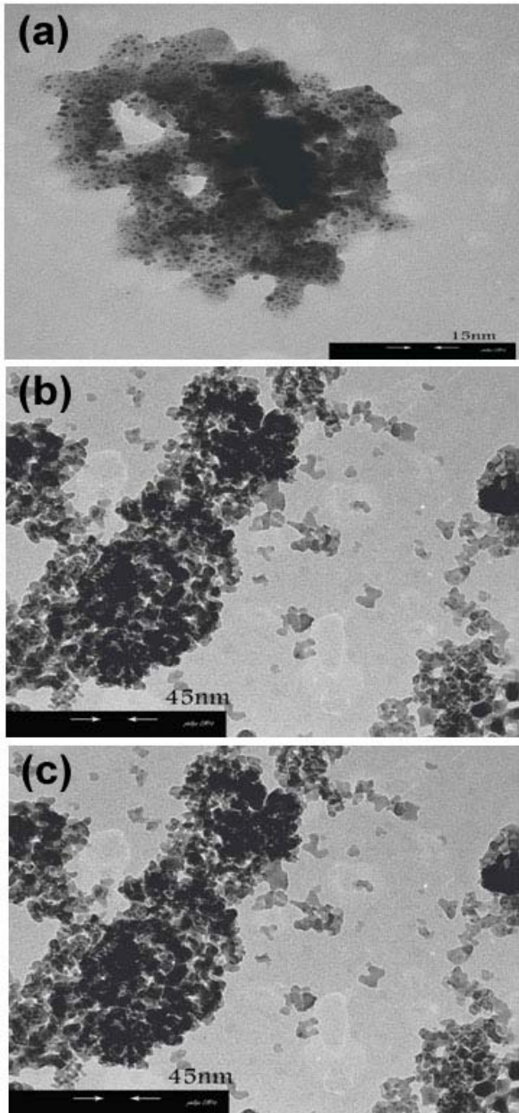
Fig. 3. Transmission electron micrograph of platinum nanoparticles dispersed on silica (a) Pt/SiO 2 = 0.047, (b) 0.095 and (c) 0.149.
