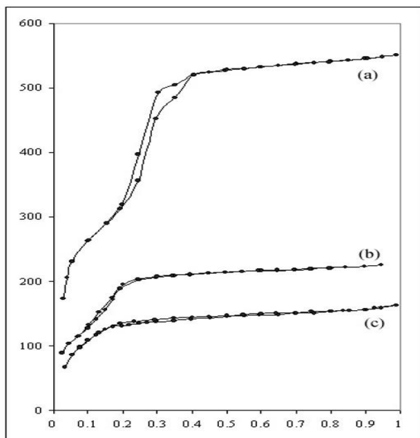
Fig. 3. Nitrogen sorption isotherms of (a) MCM-41, (b) AmpMCM-41 and (c) MoO 2 glycacAmpMCM-41.
