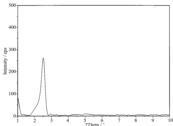
Fig. 2. X-ray diffraction pattern of MoO 2 glyacacAmpMVM-41.
