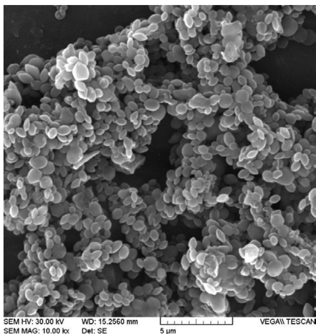
Fig. 4. SEM image of MoO 2 glycacAmpMCM-41 material.
