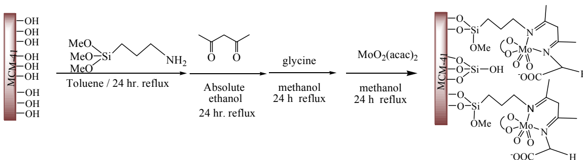
Scheme 1. Schematic illustration of MoO 2 glycacAmpMCM-41 preparation.
