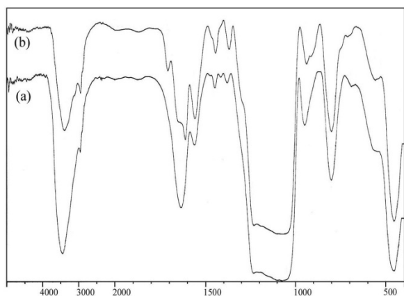
Fig. 1. FT-IR spectra of (a) glycacAmpMCM-141 and (b) MoO 2 glycacAmpMCM-41.
