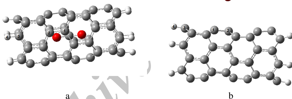
Fig. 1. Adsorption configuration of CO 2 molecule on a) inside and b) outside surface of (5, 0) nanotube.
