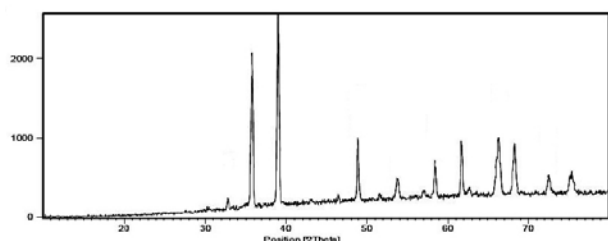
Fig. 1. The XRD pattern of copper(II) oxide nanoparticles.
