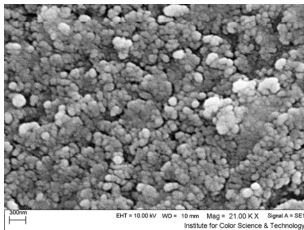
Fig. 2. SEM image of CuO nanoparticles.
