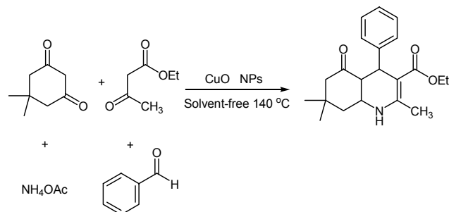
Scheme 2. The model reaction for the synthesis of polyhydroquinolines in the presence of CuO NPs.
