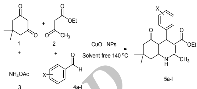
Scheme 1. Synthesis of polyhydroquinolines using CuO nanoparticles under solvent-free conditions.
