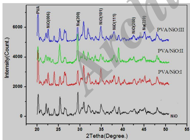
Fig. 1. XRD pattern of NiO and PVA/NiO nano hybride composite with different contents of PVA.
