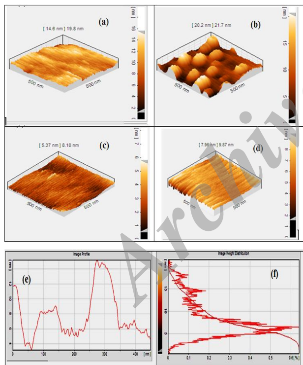
Fig. 3. AFM images (3-D) of sample (a) NiO, (b) I, (c) II and (d) III. (e)Topography spectrum as an example for sample II. (f) Particle's distribution spectrum and fitting line for sample II.
