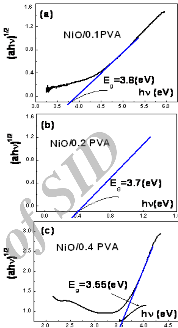
Fig.7. (a), (b) and (c) U-Spectra of PVA/NiO samples
