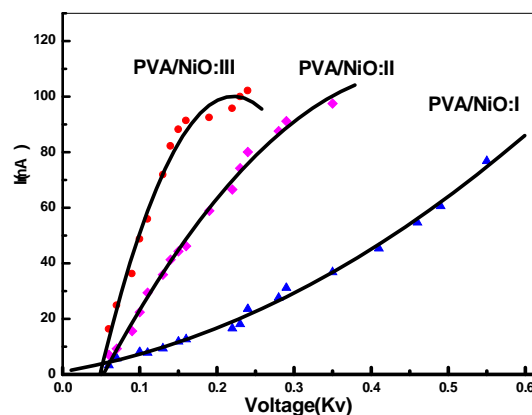
Fig.6. I-V curves of PVA/NiO samples.
