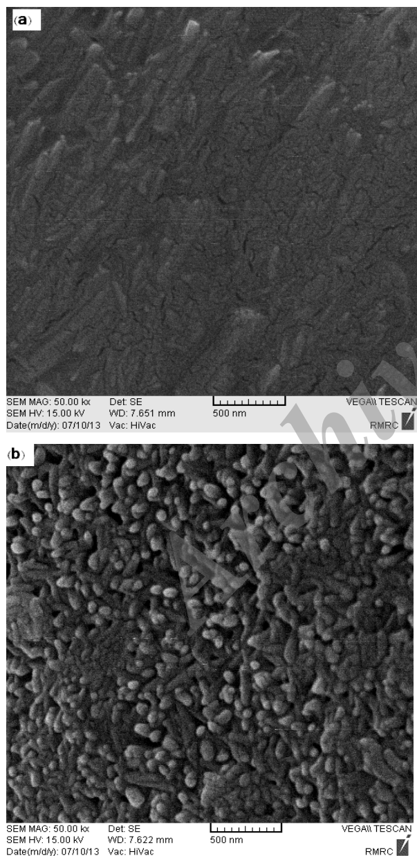
Fig. 4. SEM images of samples: (a) NiO and (b) I.
