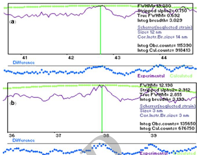
Fig. 2. The size of nano particles correspond with Fig. 1,(a) related to NiO(200) phase and (b) related to NiO(111) phase, are determined with using X- Powder soft ware.
