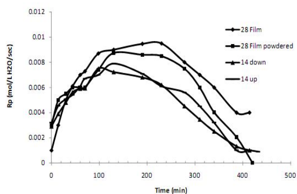
Fig. 2. Rate of polymerization ( R_p ) as a function of polymerization time.
