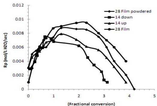
Fig. 3. Rate of polymerization ( R_p ) as a function of fractional conversion.
