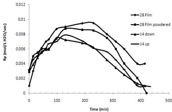
Fig. 2. Rate of polymerization ( R_p ) as a function of polymerization time.
