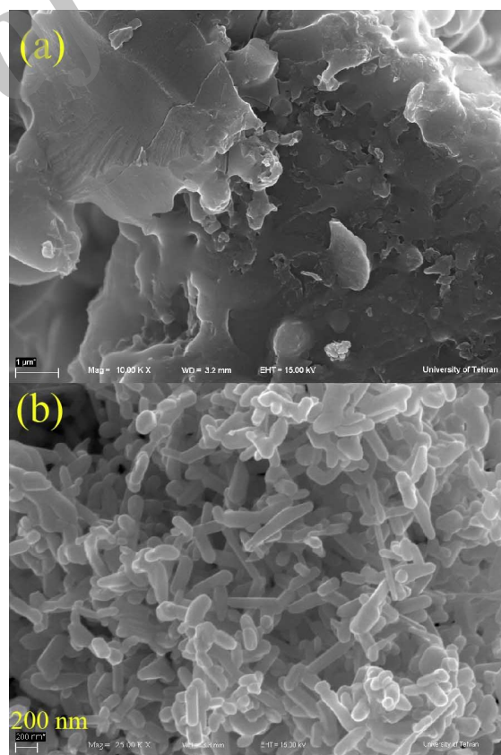
Fig. 3. SEM images of \text{Mg}(\text{OH})_2 (a) without (b) under ultrasonic waves
