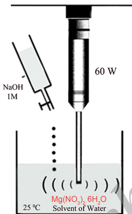
Fig. 1. Schematic diagram of preparation of \text{Mg}(\text{OH})_2 nanoparticles
