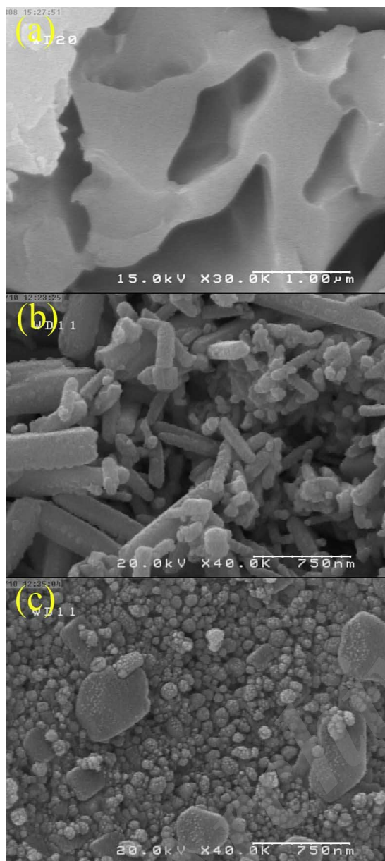
Fig. 4. SEM images of \text{Mg}(\text{OH})_2 (a) PEG (b) CTAB (c) SDBS
