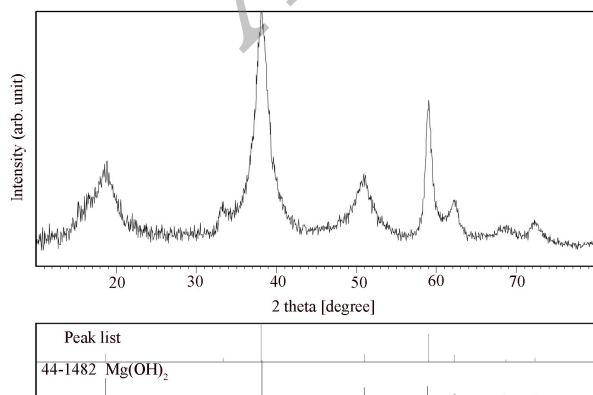
Fig. 2. XRD pattern of \text{Mg}(\text{OH})_2 nanoparticles
