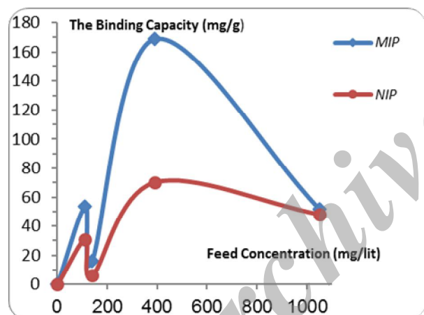
Fig. 9. The binding capacity Vs. C o
