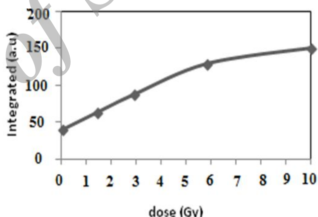
Fig. 6. Dosimetric behaviour or TL response for pure \text{CaSO}_4 exposed by gamma-ray irradiation
