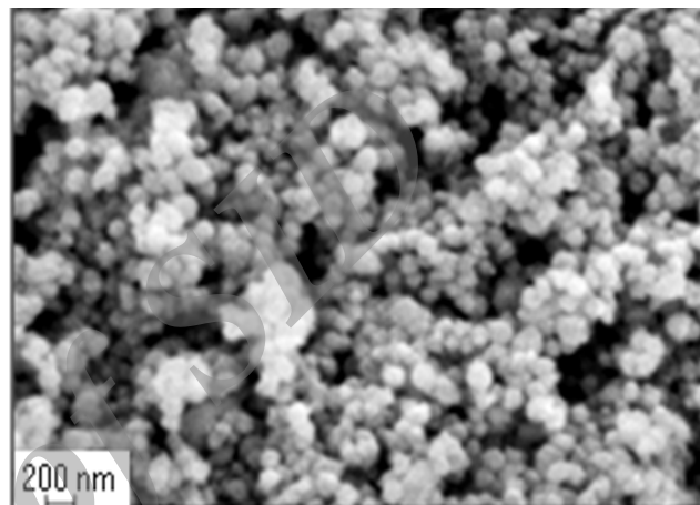
Fig. 2. SEM image of the produced CaSO 4 nanoparticles. The particles are uniform with the particles size is in conformity with that obtained from Scherrer's formula.
