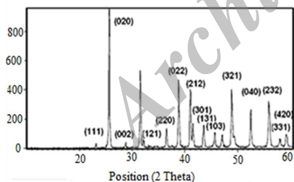
Fig. 1. XRD pattern of the pure CaSO 4 nanoparticles.
