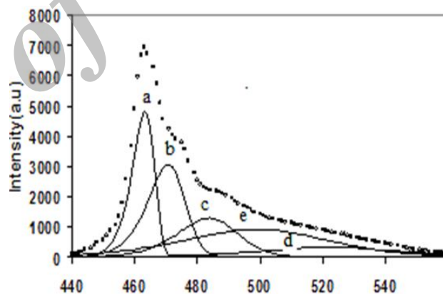
Fig. 5. TL glow curve of \text{CaSO}_4 nanoparticles I (open circles) and component glow peaks (solid lines)
