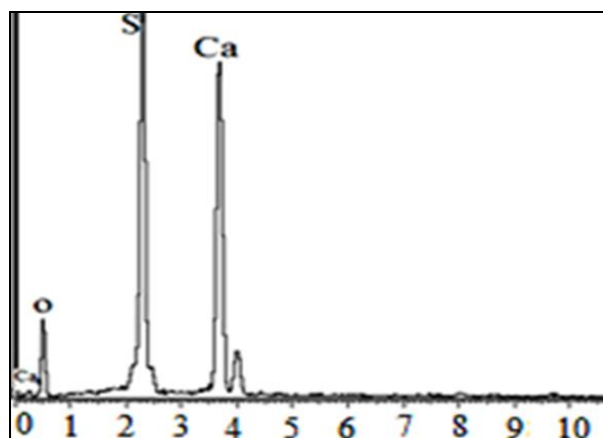
Fig. 3. EDS spectra of synthesized CaSO 4 nanoparticles
