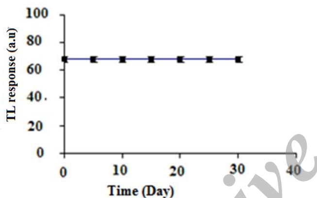
Fig. 7. TL fading of pure CaSO 4 nanocrystals exposed to 5Gy of \gamma -irradiation.
